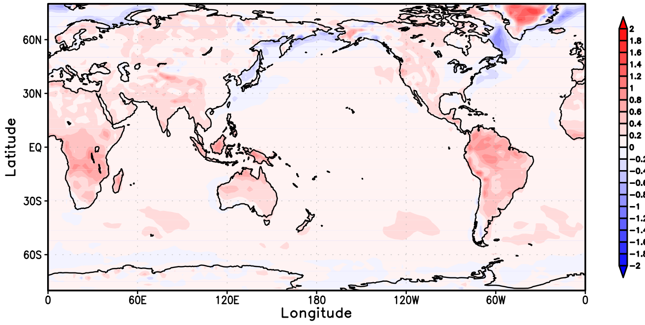
Temperature (degree) of (Nudged CAM (0.5) - GEOS) at 992hPa
